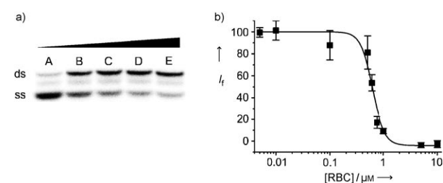
Figure 2. RBC inhibits the DNA unwinding activities of the SCV helicase. a) Titration of the duplex (ds)DNA-unwinding activity of the SARS helicase with increasing concentrations of RBC observed by radiography of the labeled duplex after acrylamide gel electrophoresis. The lower band, shown the strongest in lane A, represents the (labeled) released single-stranded (ss) DNA, whilst the upper band, shown the strongest in lane E, represents the duplex DNA. Lane A, no RBC; lanes B to E: 0.25, 0.50, 1.0, and 2.5 \mu\text{M} RBC, respectively. b) Titration of the dsDNA-unwinding activity of the SCV helicase with increasing concentrations of RBC as observed by a novel FRET assay. The data are expressed as a percentage of the control reaction in the absence of inhibitor. I_f = Cy3 relative fluorescence.
